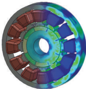
Magnetic flux density distribution in a BLDC motor
