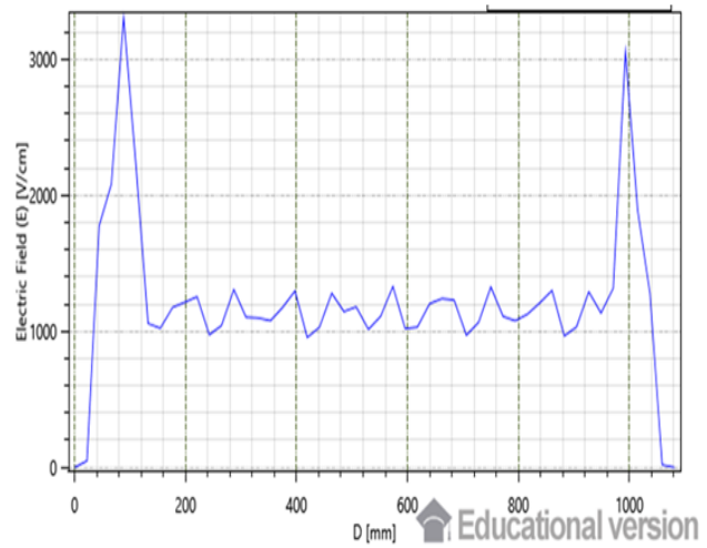
Fig 6: Electric Field distribution for 132kV Composite Long Rod Insulator
