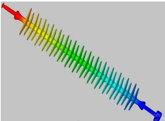
Fig 10: 3D Potential plot for 132kV Composite Long Rod Insulator
