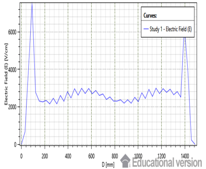
Fig 8: Electric Field distribution for 400kV Composite Long Rod Insulator
