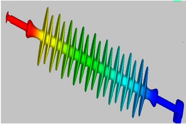
Fig 9: 3D Potential plot for 66kV Composite Long Rod Insulator
