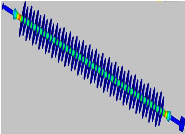
Fig 4: 3D Electric field plot for 400kV Composite Long Rod Insulator
