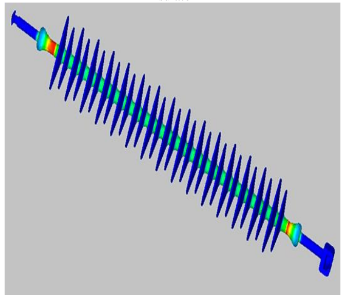
Fig 2: 3D Electric field plot for 132kV Composite Long Rod Insulator
