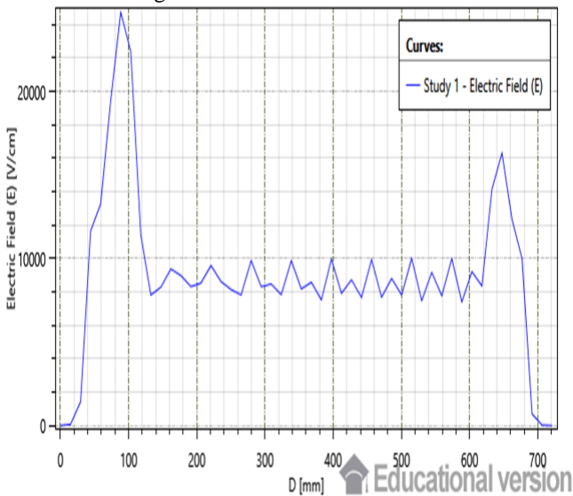
Fig 5: Electric Field distribution for 66kV Composite Long Rod Insulator
