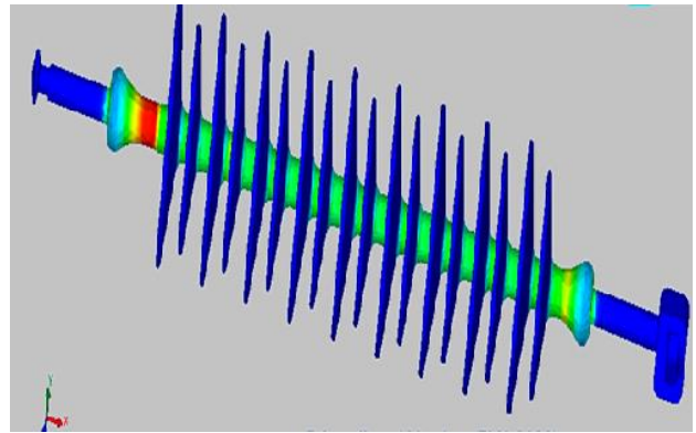
Fig 1: 3D Electric Field Plot for 66kV Composite Long Rod Insulator
